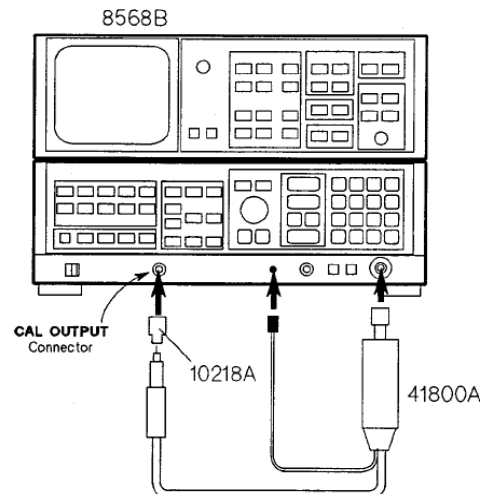
Operating Check Setup Using a Spectrum Analyzer
