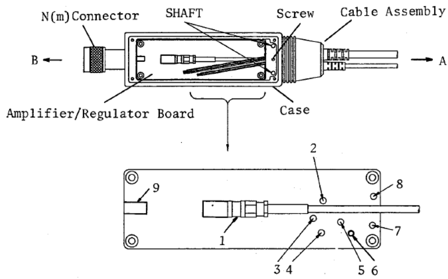
Figure 6-2 Amplifier/Regulator Board Disassembly
