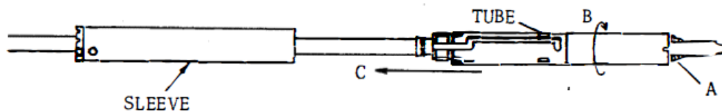
Figure 6-7 Tube Removal
