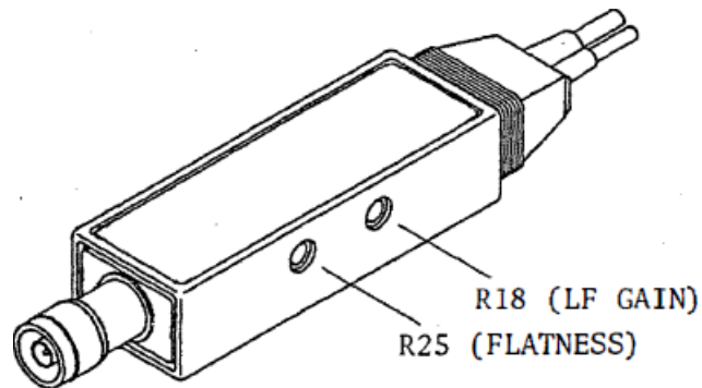
Figure 5-3 Adjustment Example
