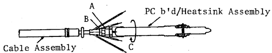
Figure 6-9 PC Board/Heatsink Assembly Removal
