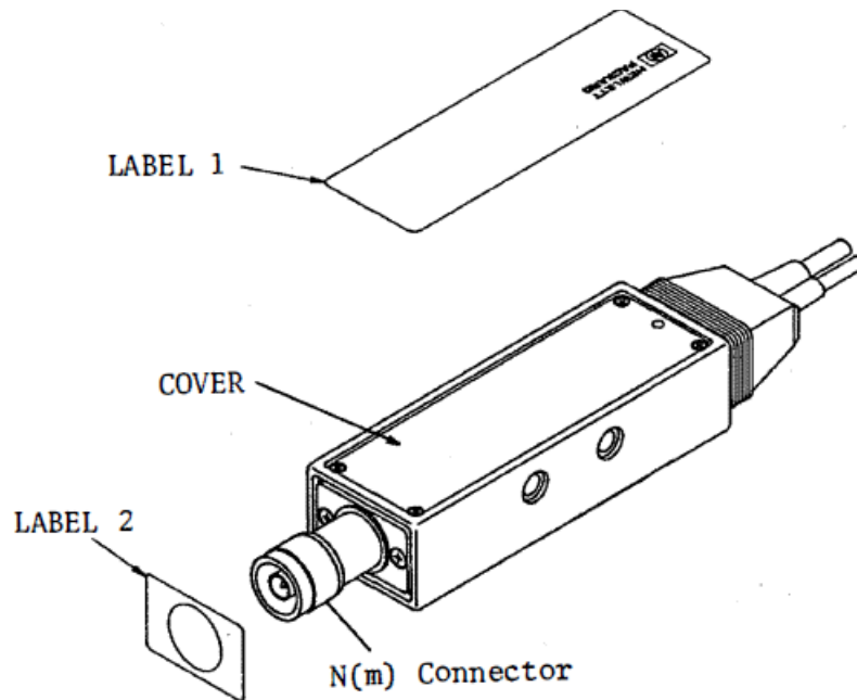
Figure 6-1 Label/Cover Removal
