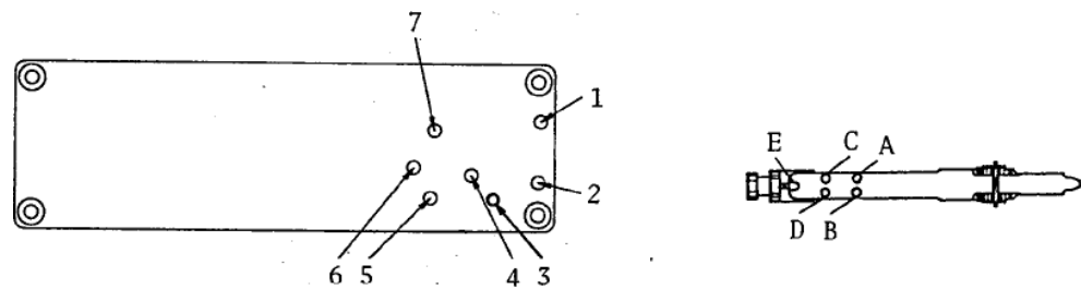
Figure 6-11 Lead Assignment
