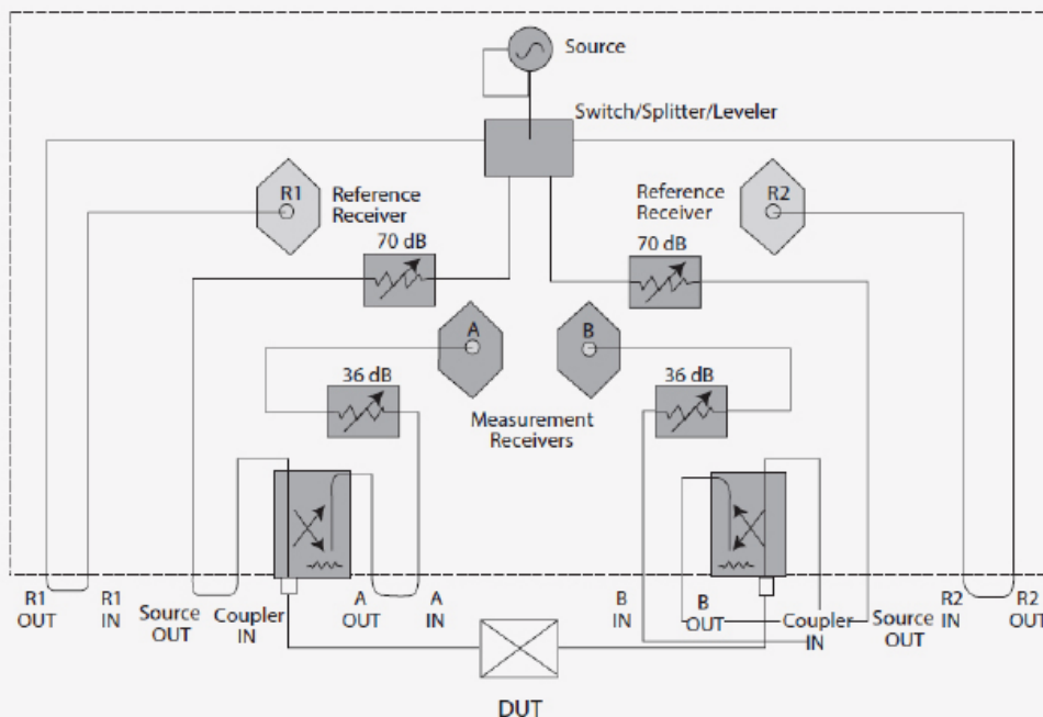
Figure 13. High dynamic range configuration that allows both forward and reverse measurements
