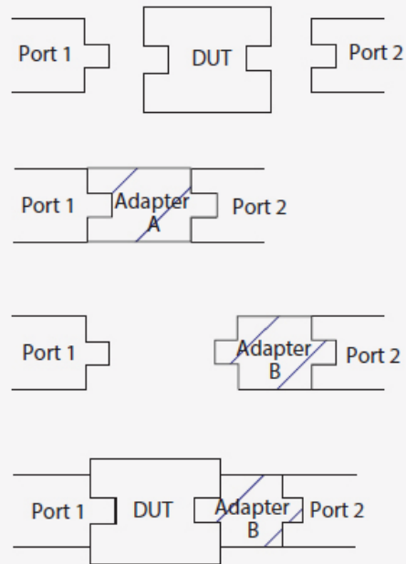
Figure 8. Swap-equal-adapters method
