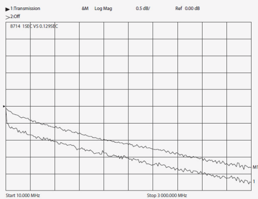
Figure 4. Reduce measurement error by increasing swap time
