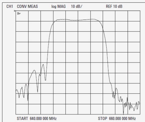
Figure 7B. High dynamic range conversion loss measurement (left) and high dynamic range setup (right)
