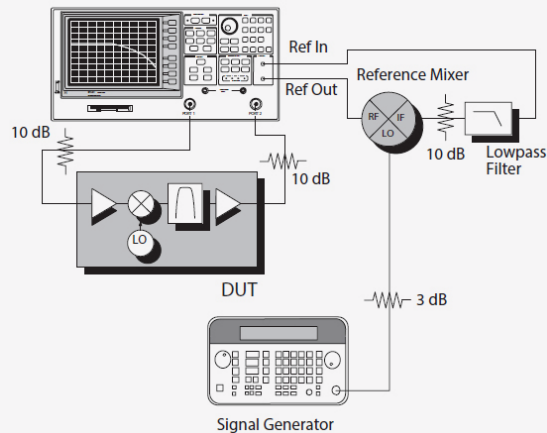
Figure 7B. High dynamic range conversion loss measurement (left) and high dynamic range setup (right)
