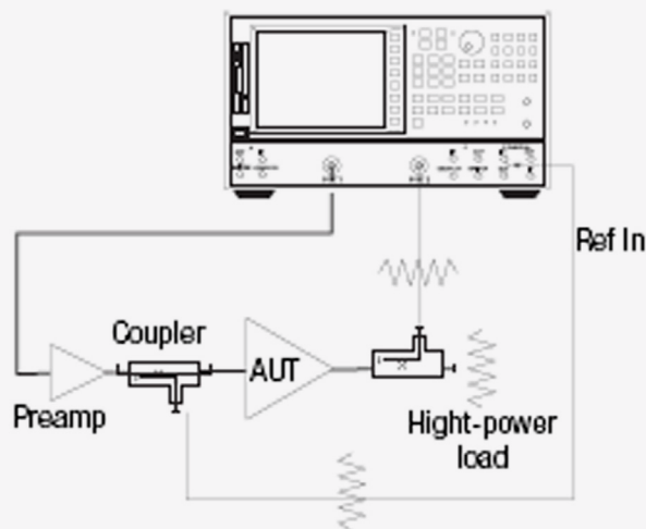
Figure 2. High-powered forward measurement configuration
