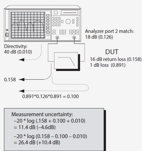
Figure 6A. Reflection measurement uncertainty
