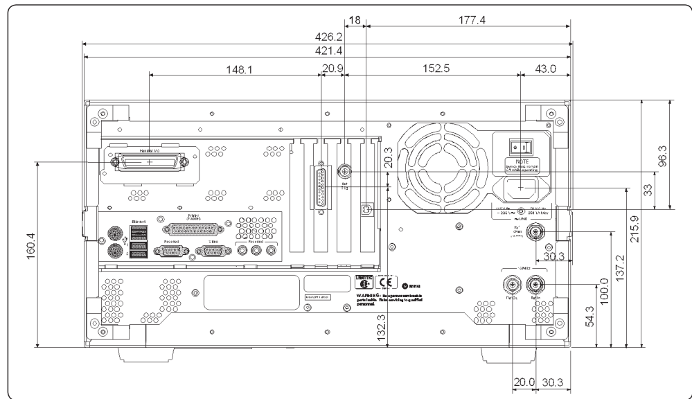
Figure 1-3. Dimensions (side view, in millimeters, nominal)
