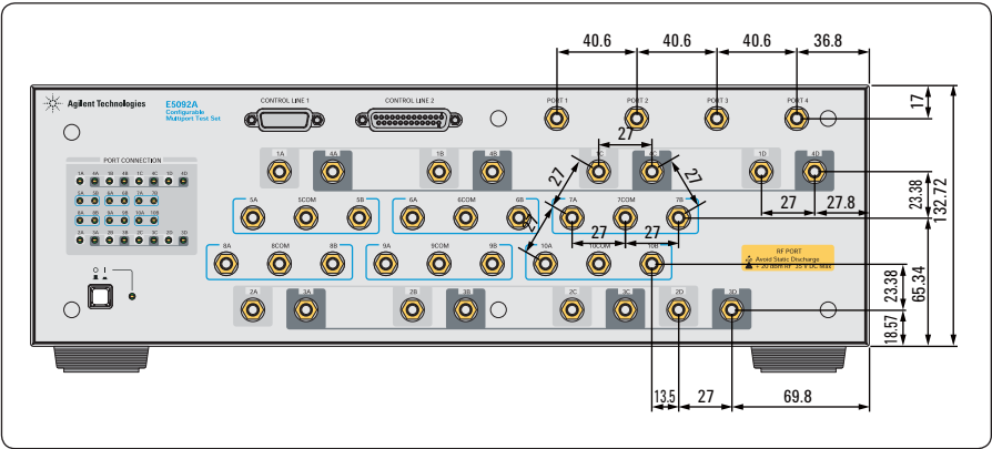
Figure 3-2. Dimensions (pitch between switches, with Option E5092A-020, in millimeters, nominal)
