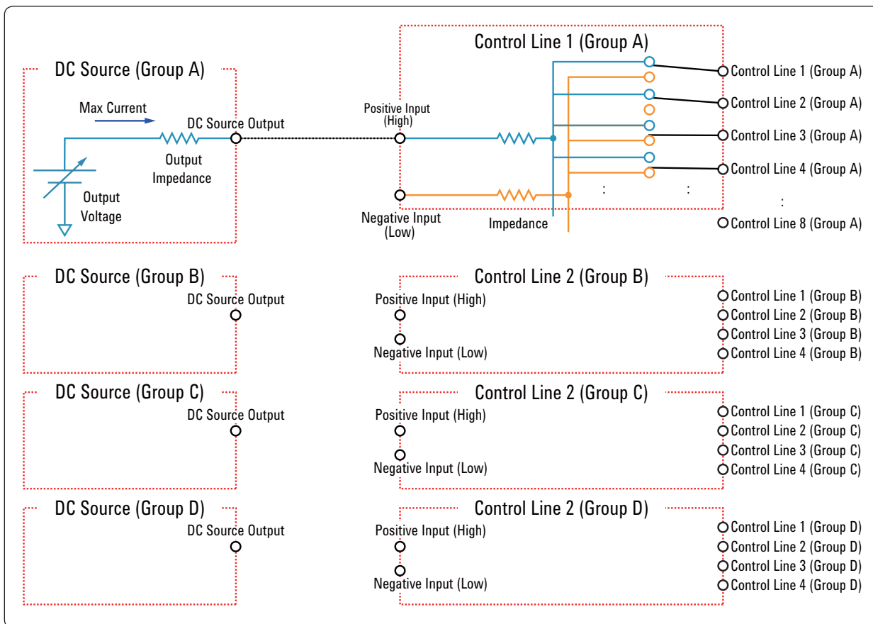
Figure 3-6. DC control line (E5092A-020)
