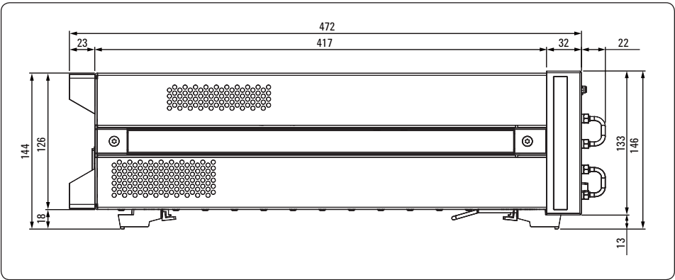
Figure 3-4. Dimensions (side view, with Option E5092A-020, in millimeters, nominal)
