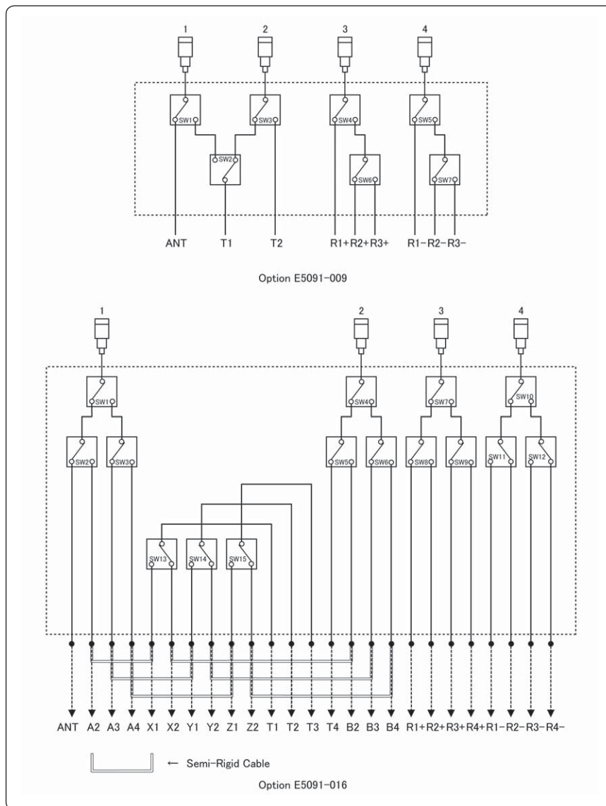
Figure 2-6. Block diagram
