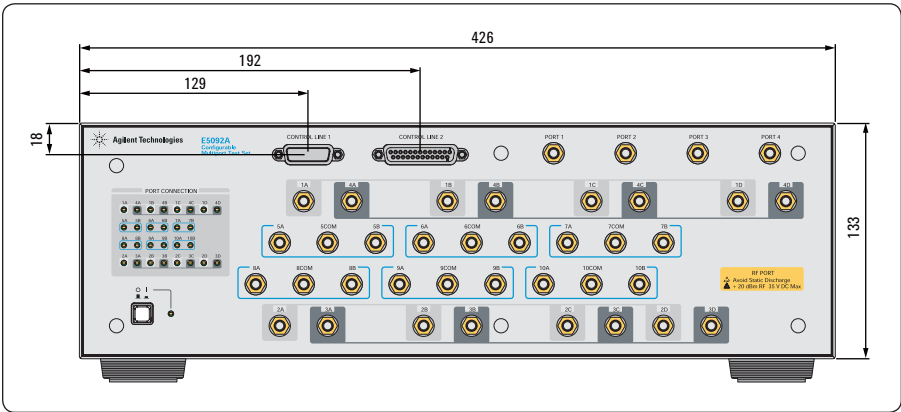
Figure 3-1. Dimensions (front view, with Option E5092A-020, in millimeters, nominal)
