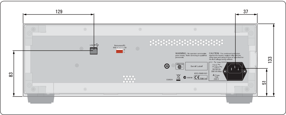
Figure 3-3. Dimensions (rear view, with Option E5092A-020, in millimeters, nominal)
