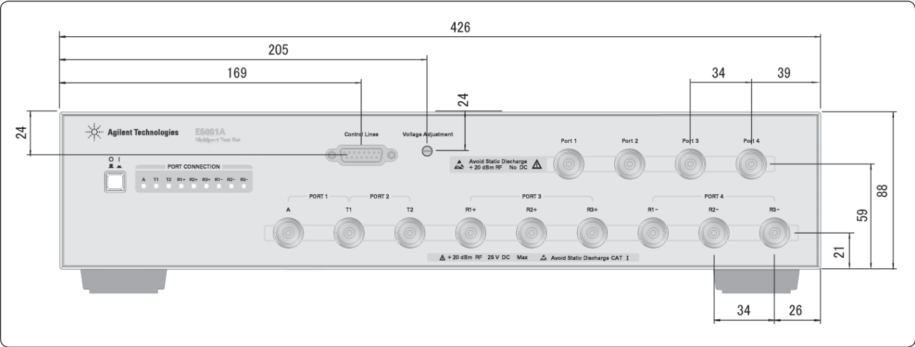
Figure 2-1. Dimensions (front view, with option E5091A-009, in millimeters, nominal)
