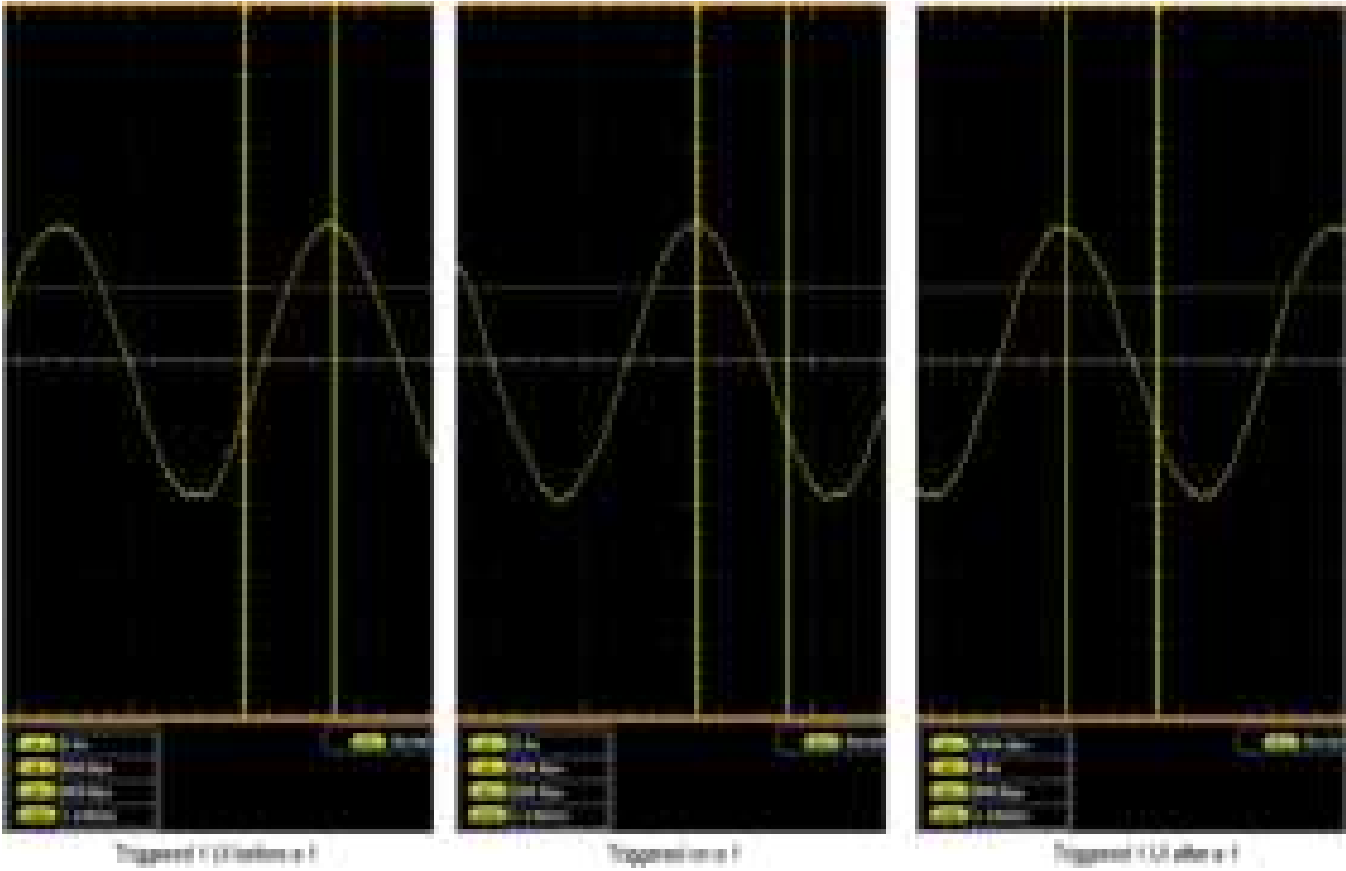
Figure 43: Isolated 1 triggering
