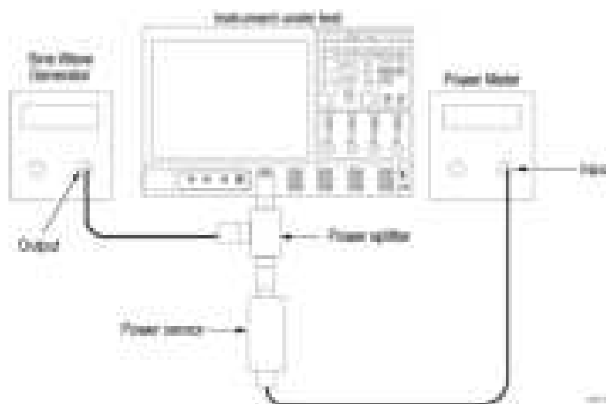
Figure 46: Sine wave generator leveling equipment setup
