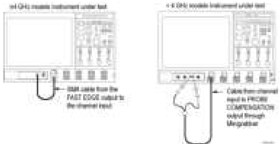
Figure 5: Setup for trigger test
