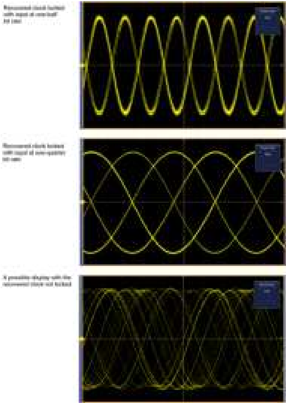
Figure 45: Clock recovery
