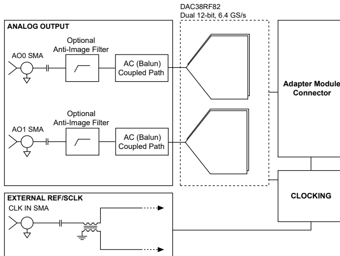
Figure 1. PXle-5745 Block Diagram
