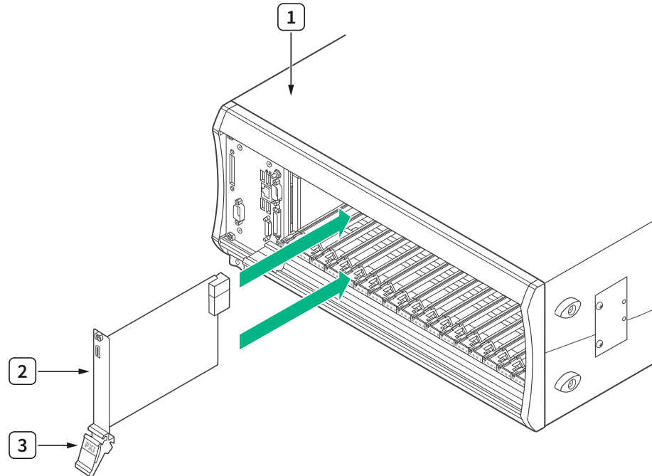
Figure 2. Module Installation
