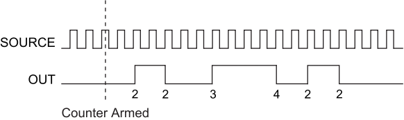
Figure 75. Finite Implicit Buffered Pulse Train Generation
