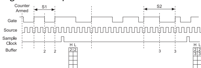
Figure 53. Sample Clocked Buffered Pulse Measurement
