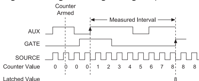
Figure 66. Single Two-Signal Edge-Separation Measurement
