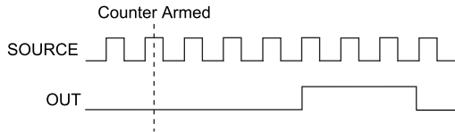
Figure 69. Single Pulse Generation
