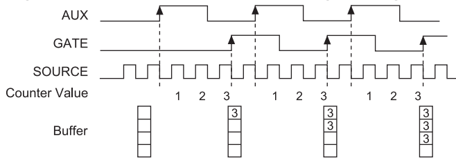
Figure 67. Implicit Buffered Two-Signal Edge-Separation Measurement
