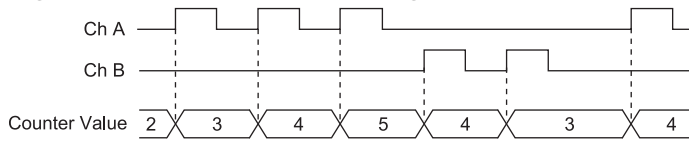
Figure 64. Measurements Using Two Pulse Encoders
