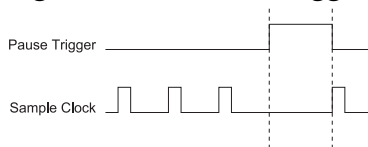
Figure 35. AO Pause Trigger with the Onboard Clock Source
