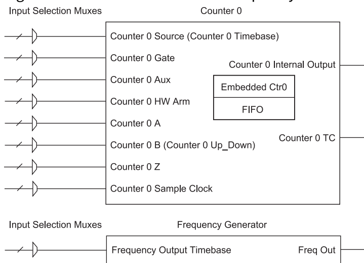
Figure 44. Chassis Counter 0 and Frequency Generator
