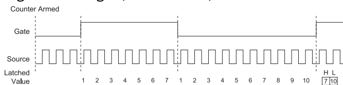
Figure 51. Single (On-Demand) Pulse Measurement
