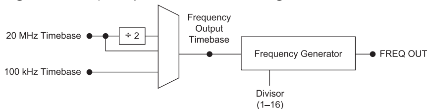
Figure 77. Frequency Generator Block Diagram
