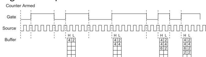
Figure 52. Implicit Buffered Pulse Measurement
