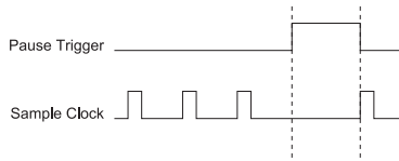
Figure 41. DO Pause Trigger with the Onboard Clock Source
