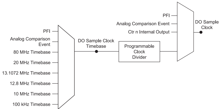
Figure 40. Digital Output Timing Options
