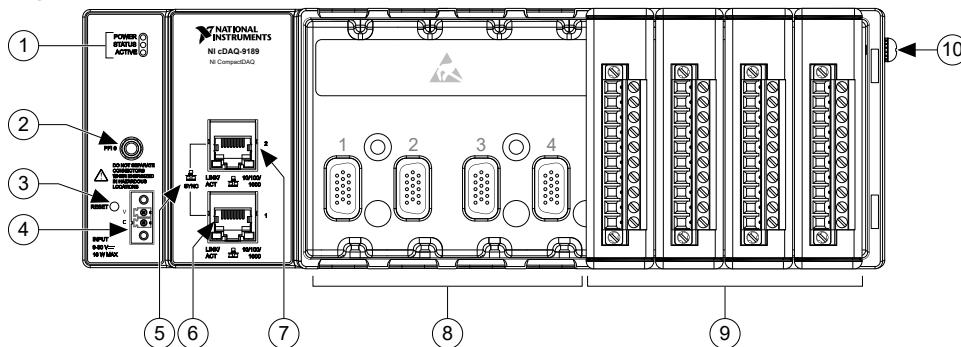
Figure 3. cDAQ-9189 Front Panel
