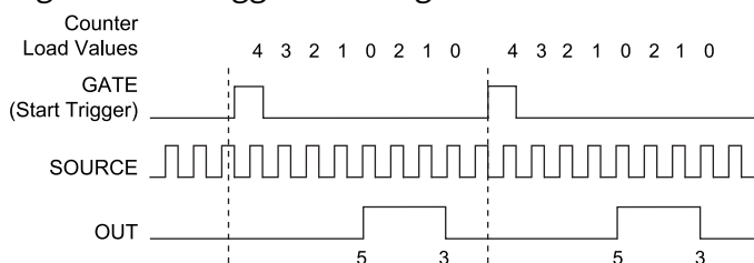
Figure 72. Retriggerable Single Pulse Generation with Initial Delay on Retrigger
