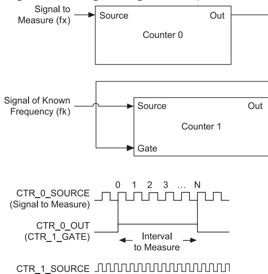
Figure 57. Large Range of Frequencies with Two Counters
