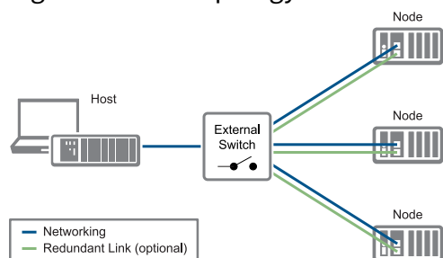
Figure 30. Star Topology
