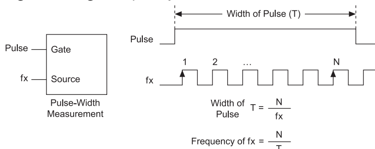
Figure 56. High Frequency with Two Counters
