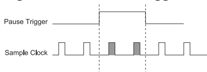
Figure 36. AO Pause Trigger with Other Signal Source
