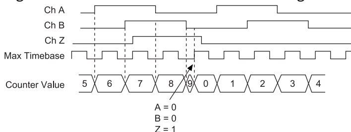
Figure 63. Channel Z Reload with X4 Decoding
