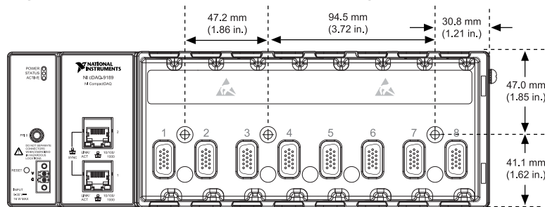
Figure 18. cDAQ-9189 Surface Mounting Dimensions (cDAQ-9189 Shown)
