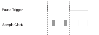
Figure 42. DO Pause Trigger with Other Signal Source
