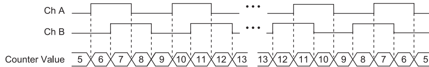
Figure 62. X4 Encoding
