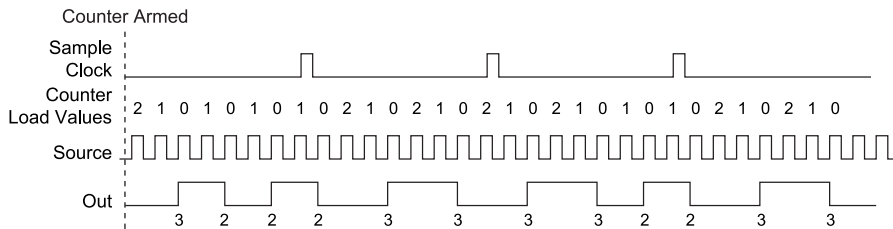
Figure 76. Finite Buffered Sample Clocked Pulse Train Generation
