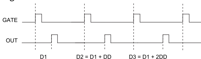
Figure 79. Pulse Generation for ETS
