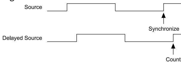
Figure 82. External or Internal Source Less than 20 MHz
