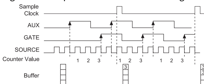
Figure 68. Sample Clocked Buffered Two-Signal Separation Measurement
