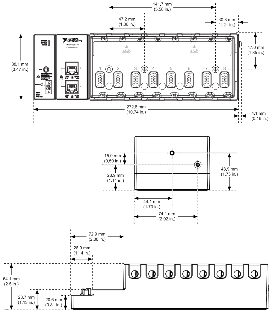
Figure 27. cDAQ-9189 Dimensions
