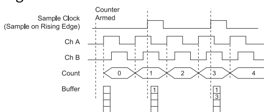
Figure 65. Buffered Position Measurement
