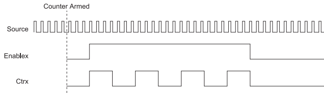
Figure 71. Finite Pulse Train Generation: Four Ticks Initial Delay, Four Pulses
