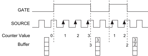
Figure 49. Implicit Buffered Pulse-Width Measurement
