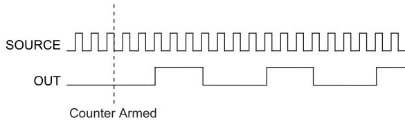
Figure 74. Continuous Pulse Train Generation
