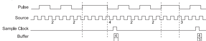
Figure 50. Sample Clocked Buffered Pulse-Width Measurement
