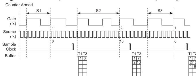
Figure 58. Sample Clocked Buffered Frequency Measurement (Averaging)
