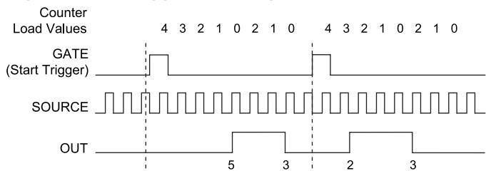
Figure 73. Retriggerable Single Pulse Generation False
