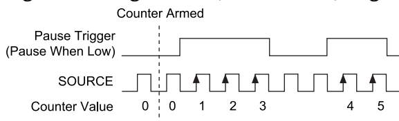
Figure 46. Single Point (On-Demand) Edge Counting with Pause Trigger
