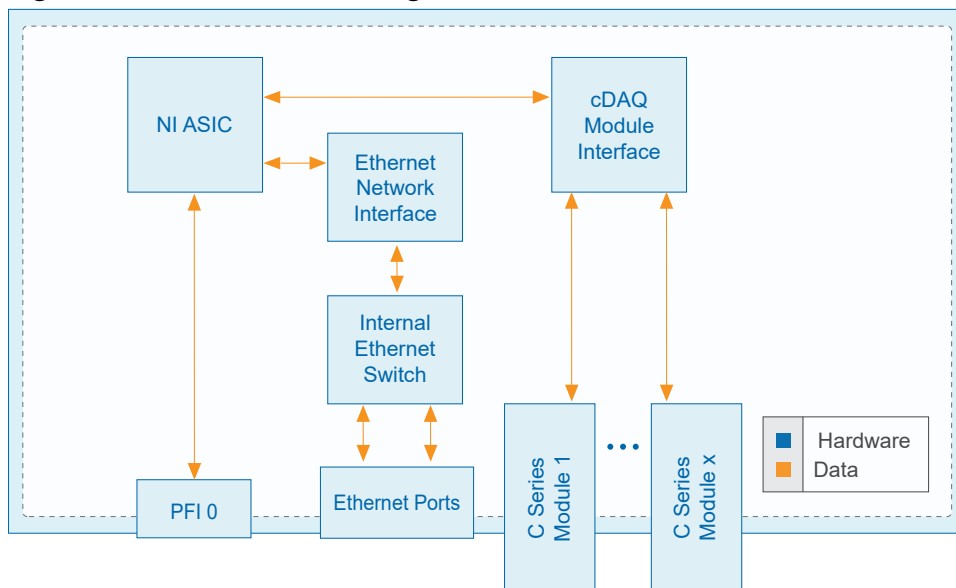
Figure 2. cDAQ-9189 Block Diagram
