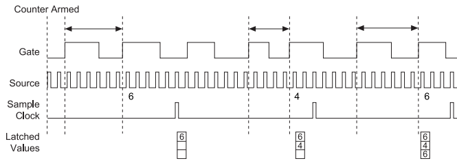
Figure 59. Sample Clocked Buffered Frequency Measurement (Non-Averaging)
