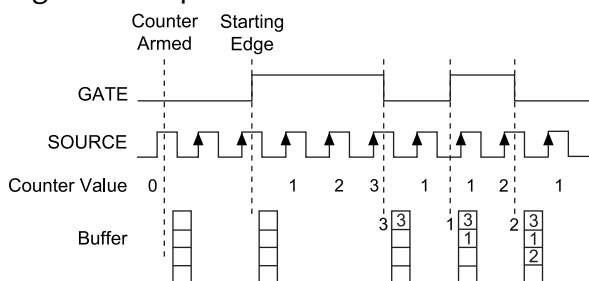
Figure 54. Implicit Buffered Semi-Period Measurement
