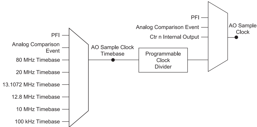
Figure 34. Analog Output Timing Options
