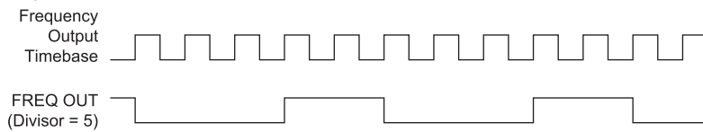
Figure 78. Frequency Generator Output Waveform
