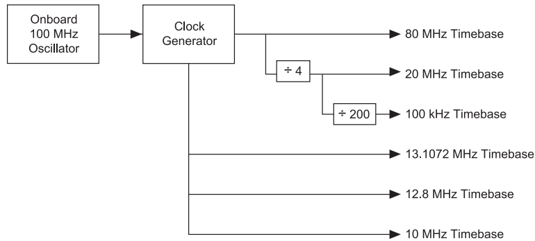
Figure 83. Clock Routing Circuitry
