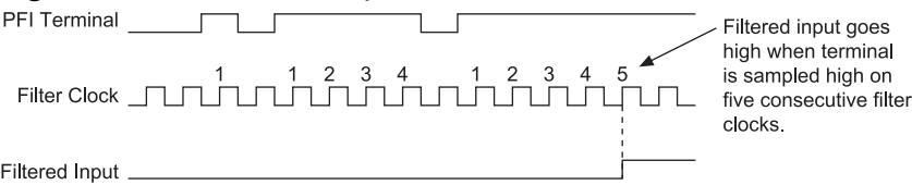
Figure 43. PFI Filter Example
