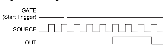
Figure 70. Single Pulse Generation with Start Trigger
