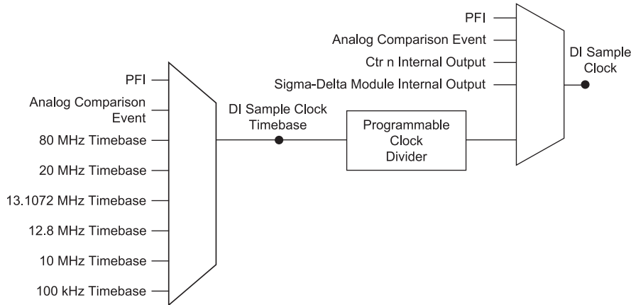
Figure 37. DI Sample Clock Timing Options
