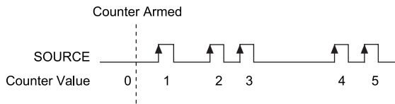
Figure 45. Single Point (On-Demand) Edge Counting
