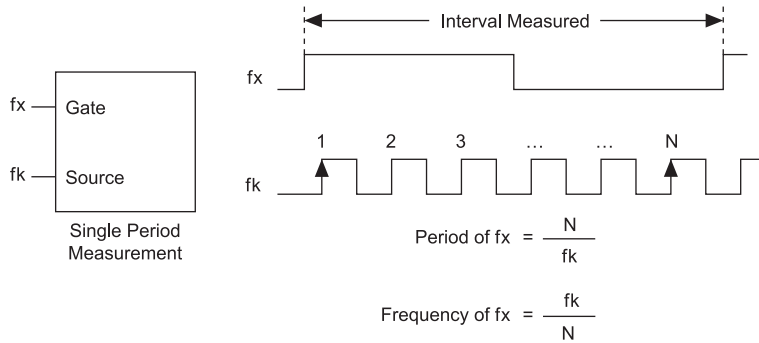
Figure 55. Low Frequency with One Counter
