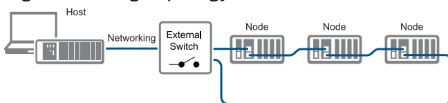
Figure 29. Ring Topology
