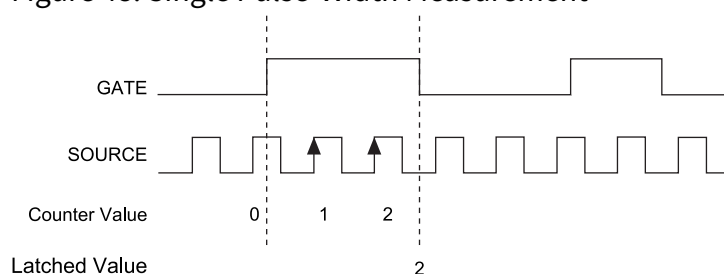
Figure 48. Single Pulse-Width Measurement
